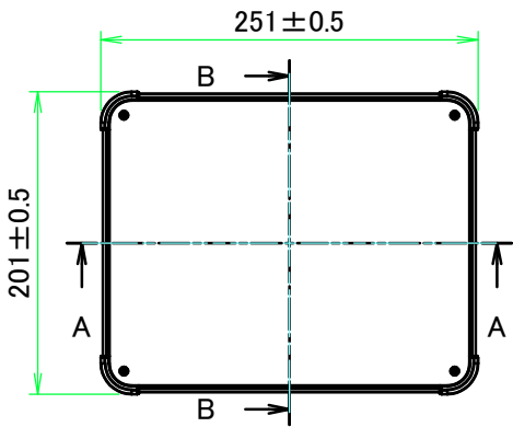
E view
